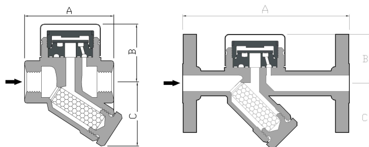
TRAP No.D80 DIMENSIONS (MM). MOP(KG/CM 2 ). WT(KG)
